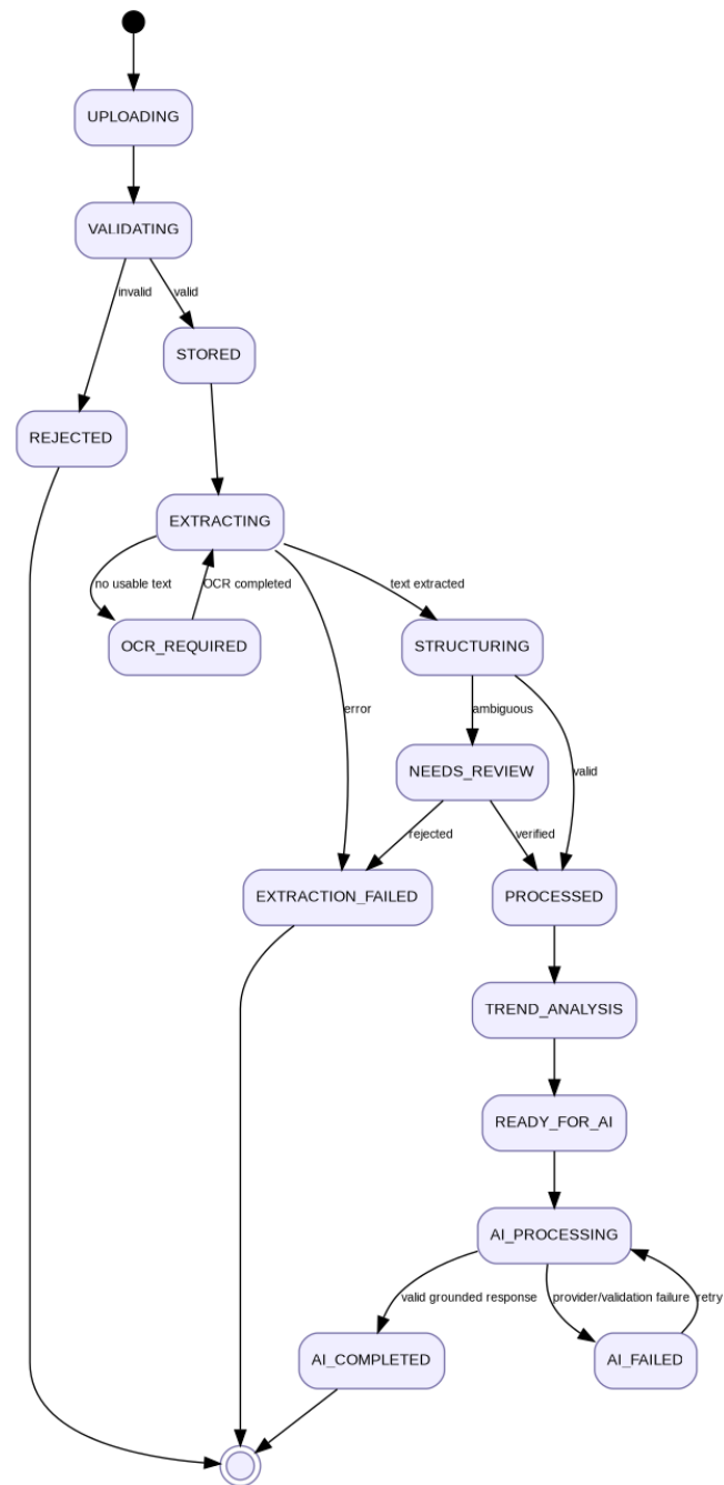
Diagram 7 — State Machine Diagram (Report Processing)
