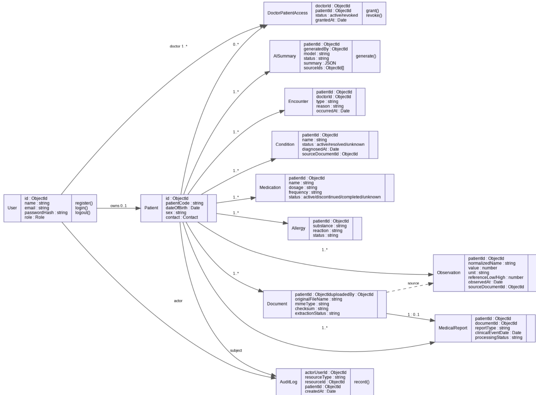
Diagram 2 — Class Diagram
